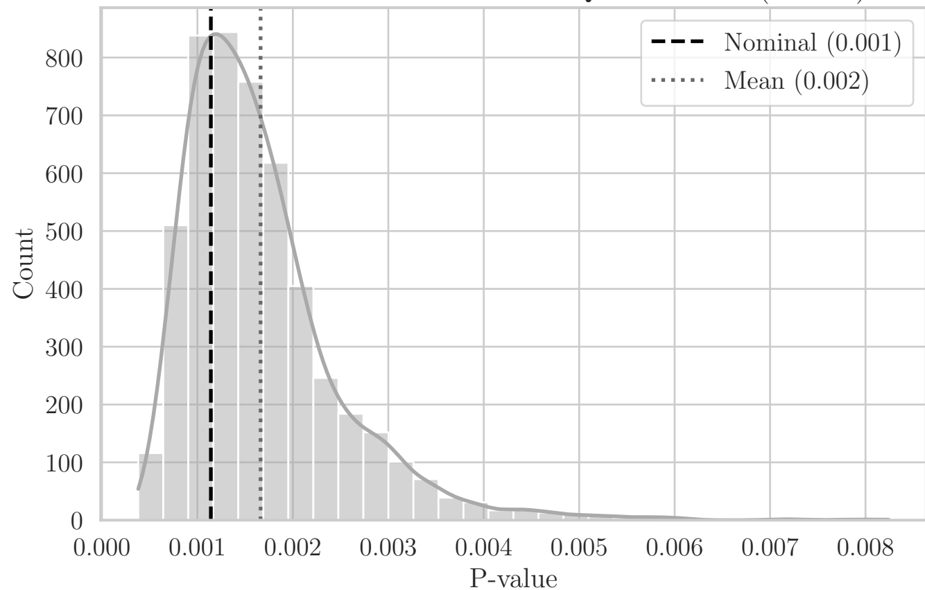
MC Distribution of P-values for QRS Distance (F2 XY)
