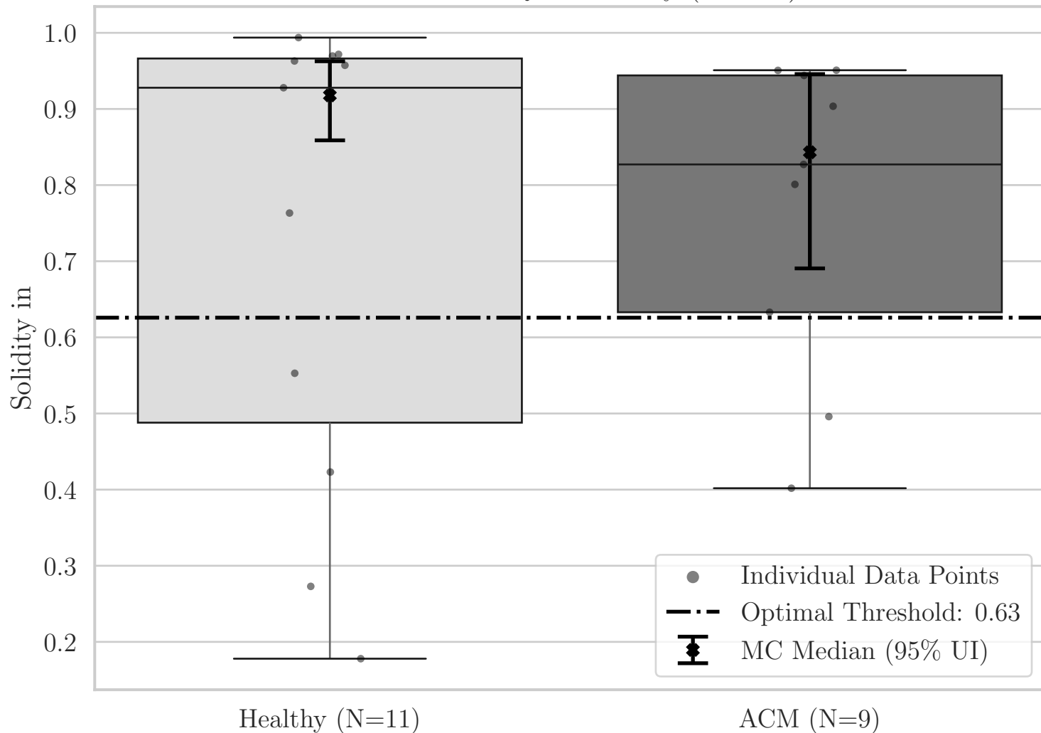
Box Plot for QRS Solidity (F2 XY)
