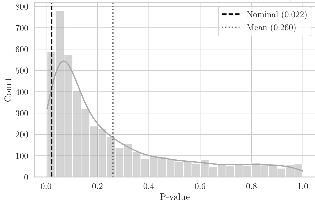
MC Distribution of P-values for ST Area_Net (F2 XY)
