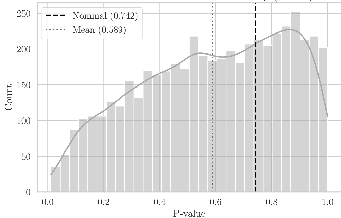
MC Distribution of P-values for ST Solidity (F2 XY)
