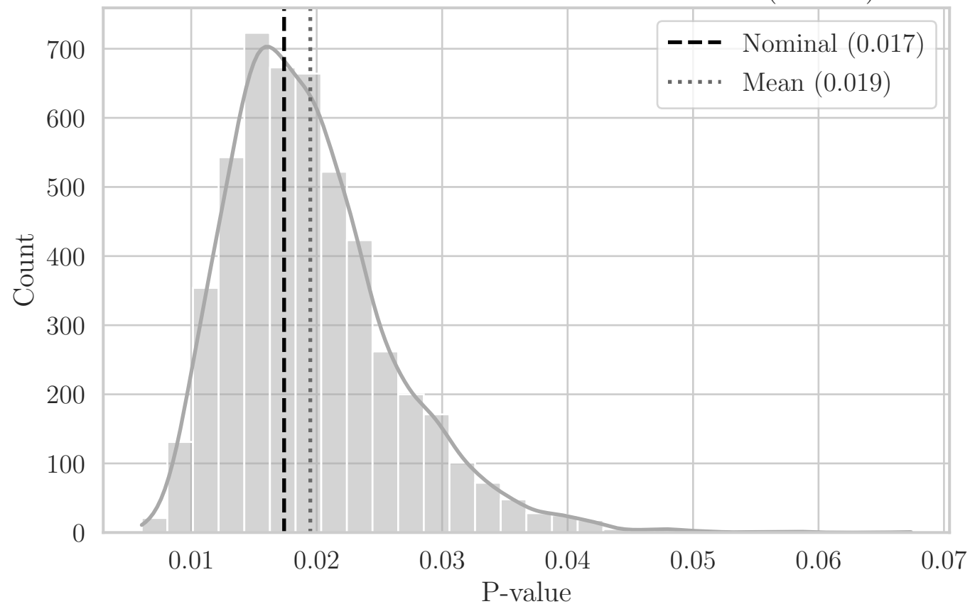
MC Distribution of P-values for T Area_Hull (F2 XY)
