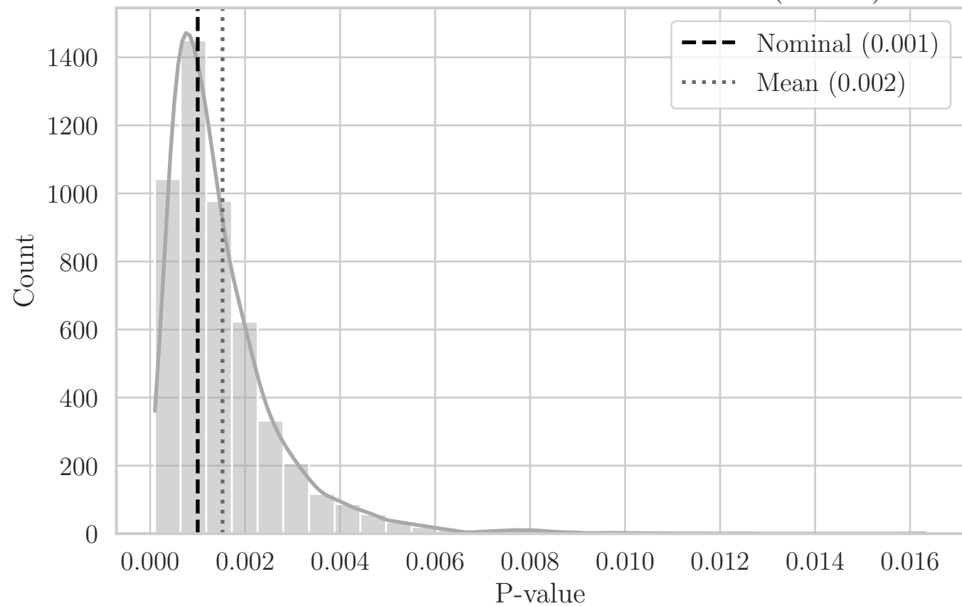
MC Distribution of P-values for T Distance (F2 XY)
