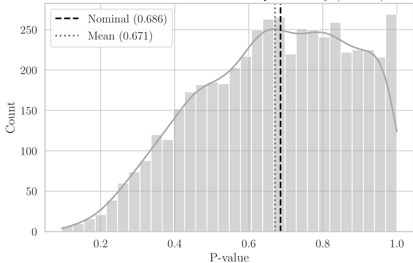
MC Distribution of P-values for QRS Solidity (NL YZ)
