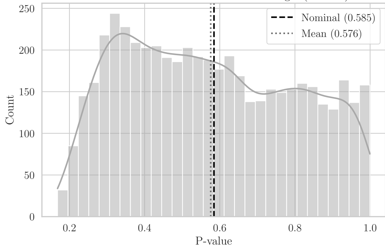
MC Distribution of P-values for ST Angle (NL YZ)
