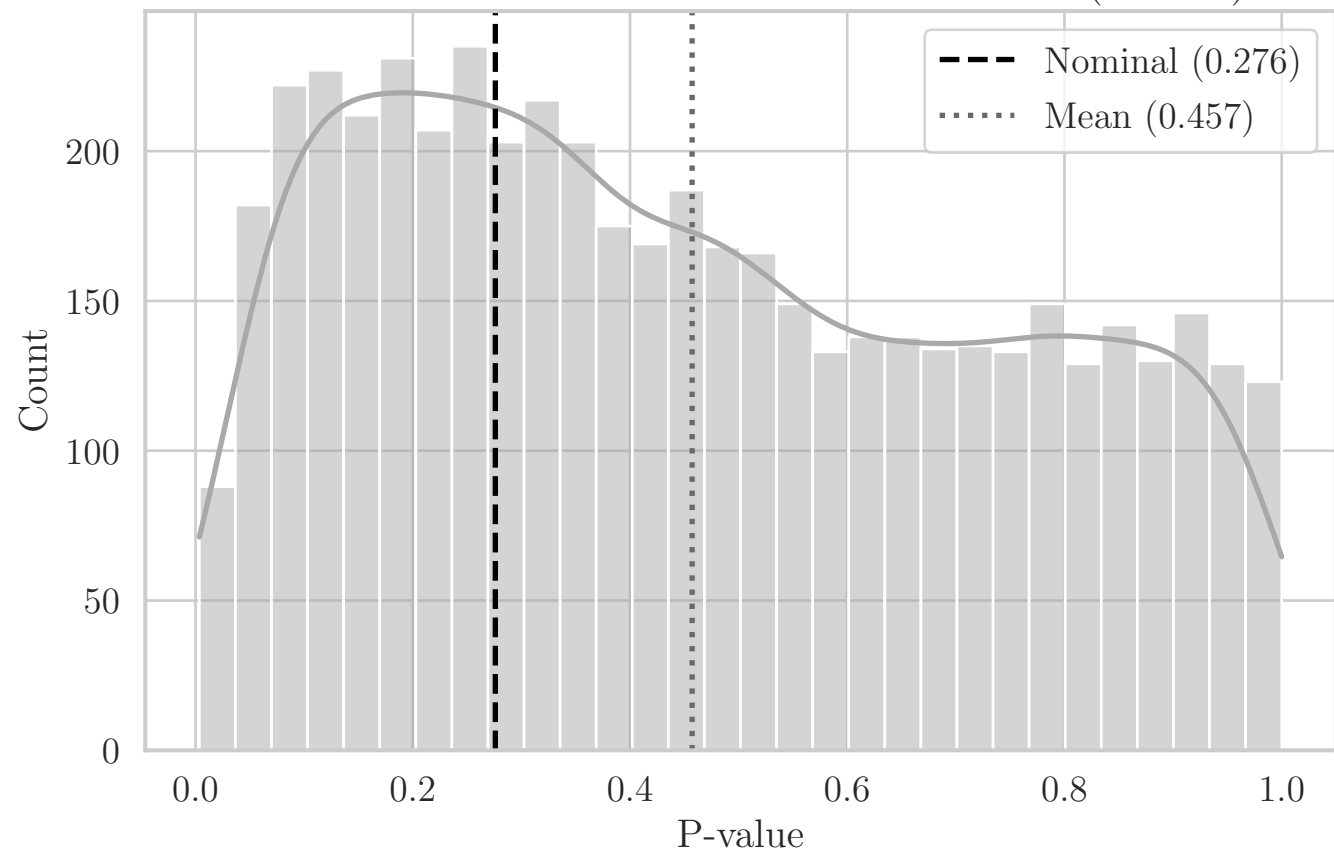
MC Distribution of P-values for ST Area_Hull (NL YZ)
