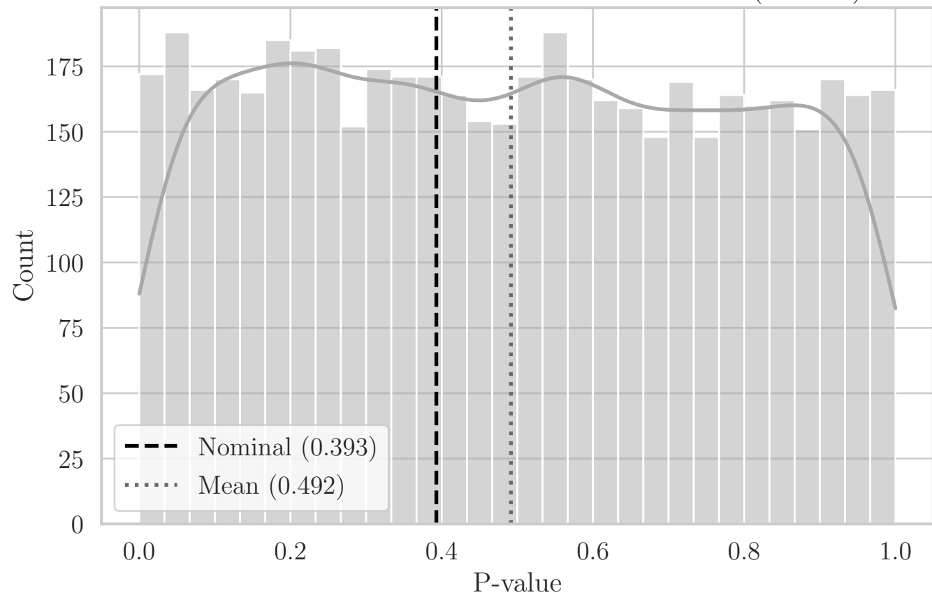
MC Distribution of P-values for ST Distance (NL YZ)
