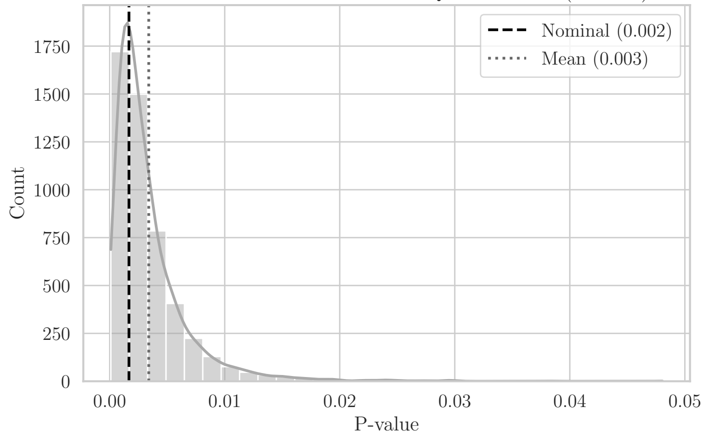
MC Distribution of P-values for QRS Distance (OO YZ)
