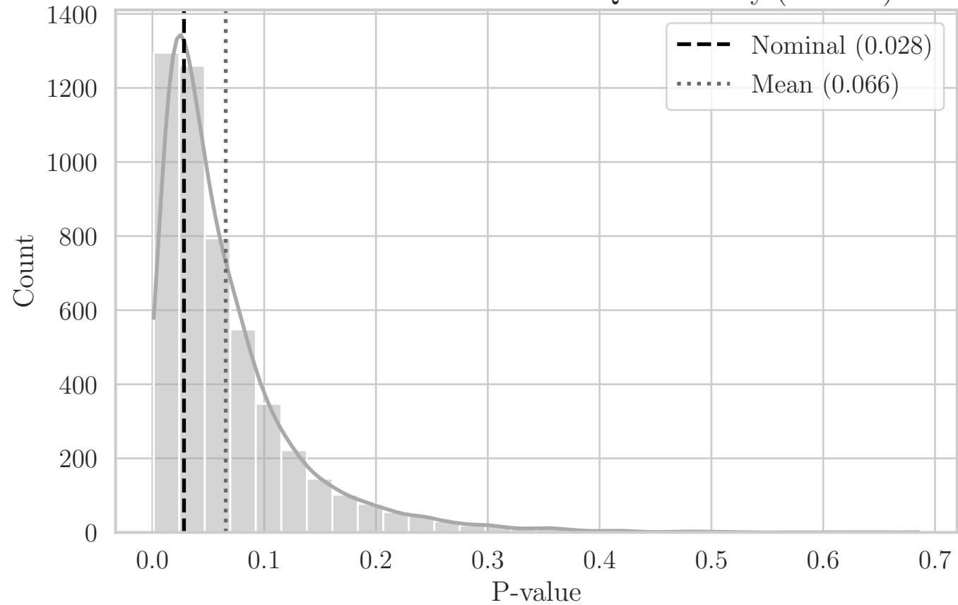
MC Distribution of P-values for QRS Solidity (OO YZ)
