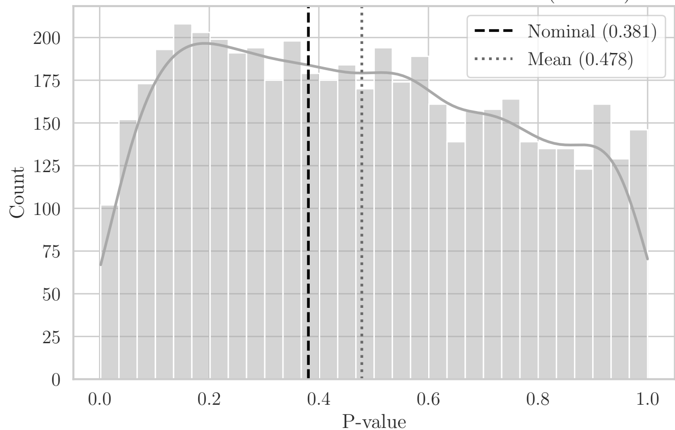
MC Distribution of P-values for ST Area_Hull (OO YZ)
