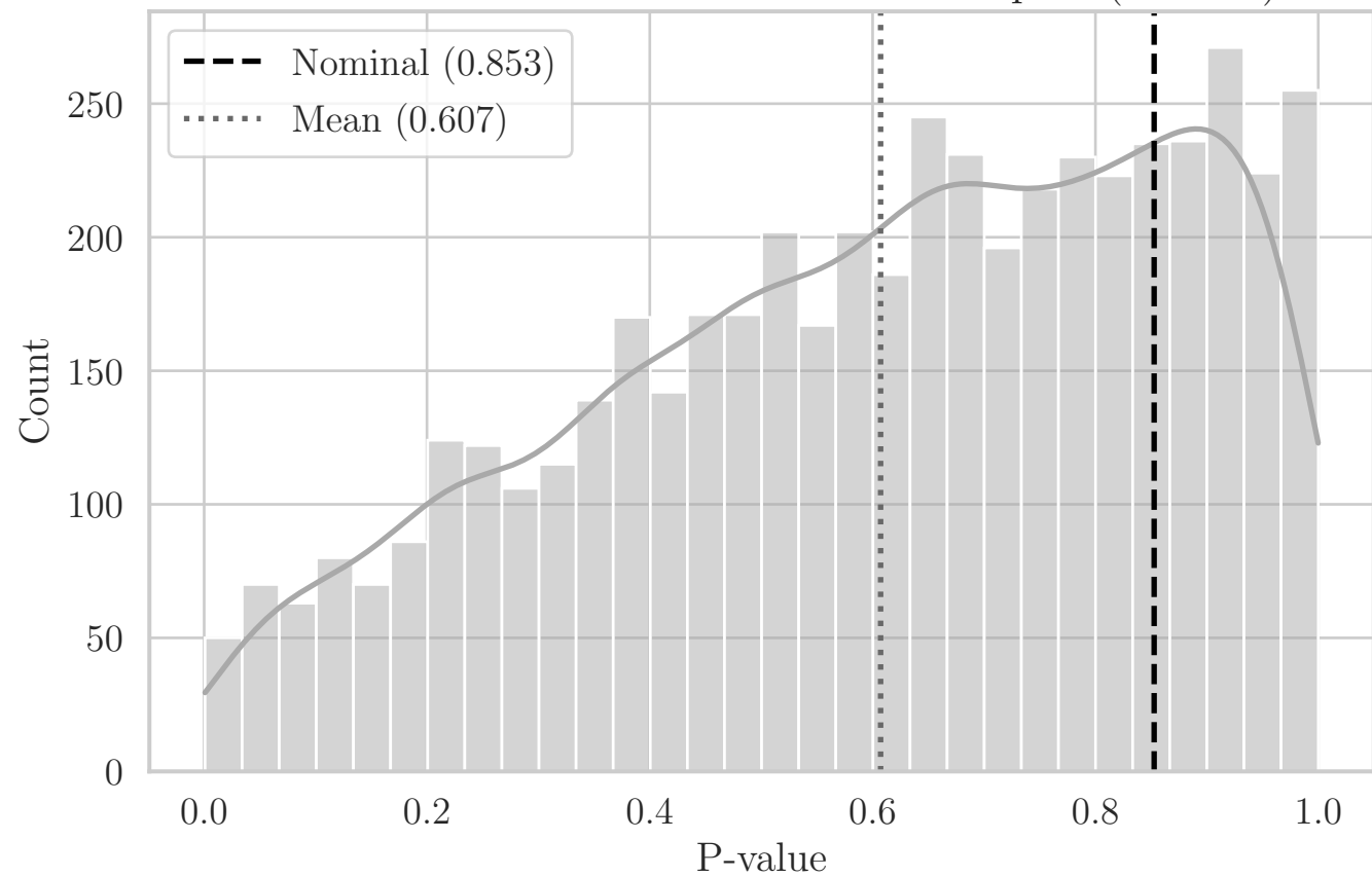
MC Distribution of P-values for ST Compact (OO YZ)
