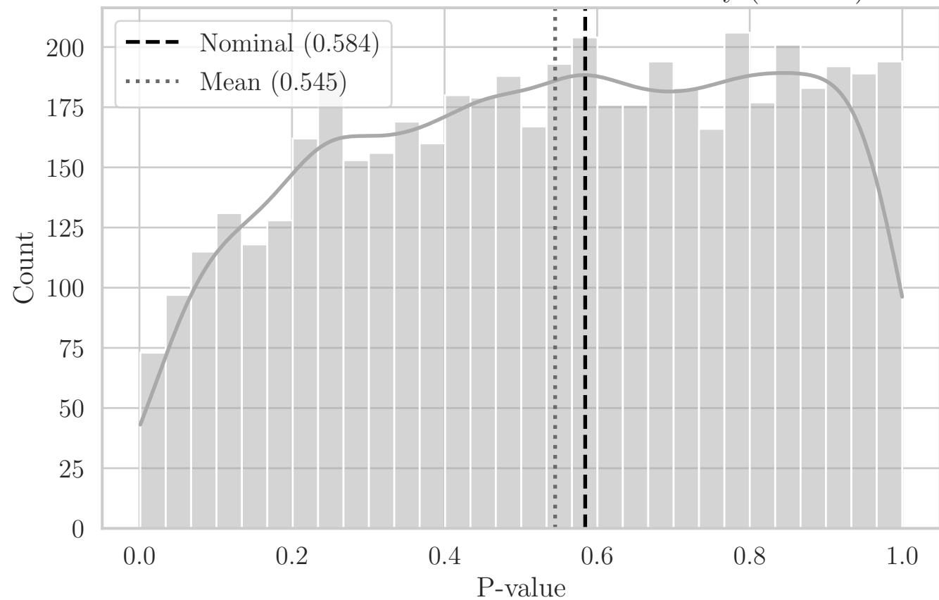
MC Distribution of P-values for ST Solidity (OO YZ)
