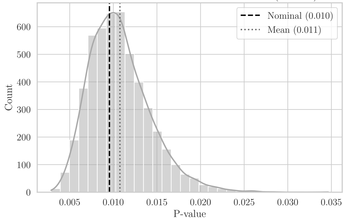
MC Distribution of P-values for T Area_Hull (OO YZ)
