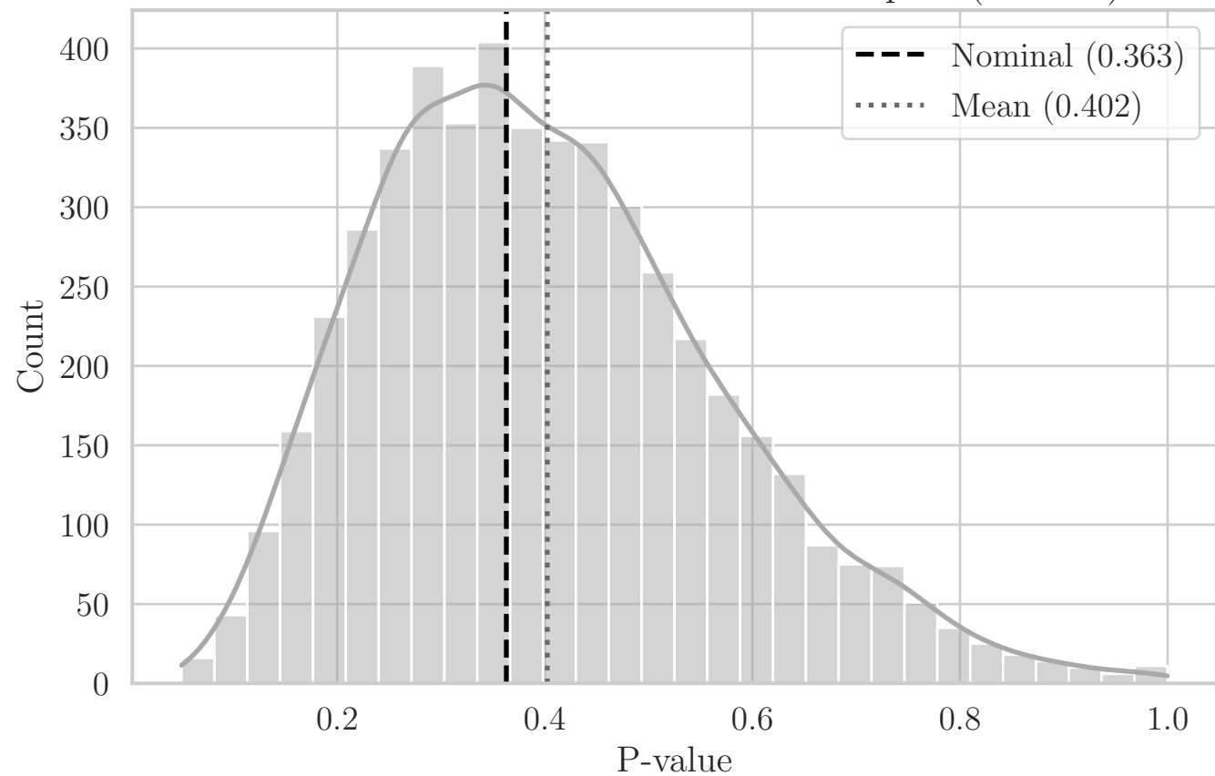
MC Distribution of P-values for T Compact (OO YZ)
