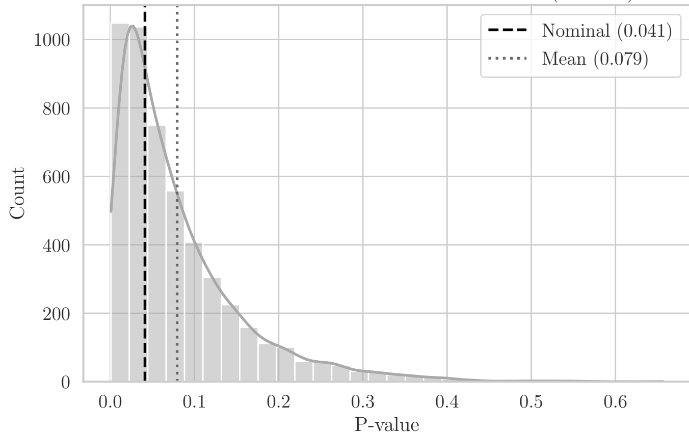
MC Distribution of P-values for T Distance (OO YZ)
