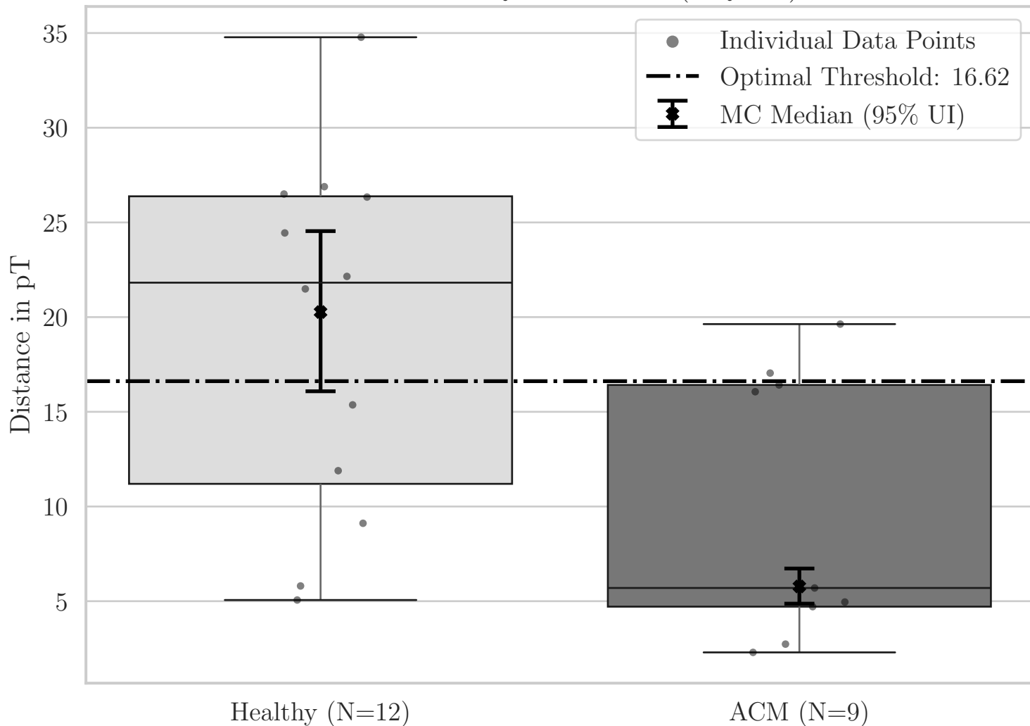
Box Plot for QRS Distance (OQ XY)
