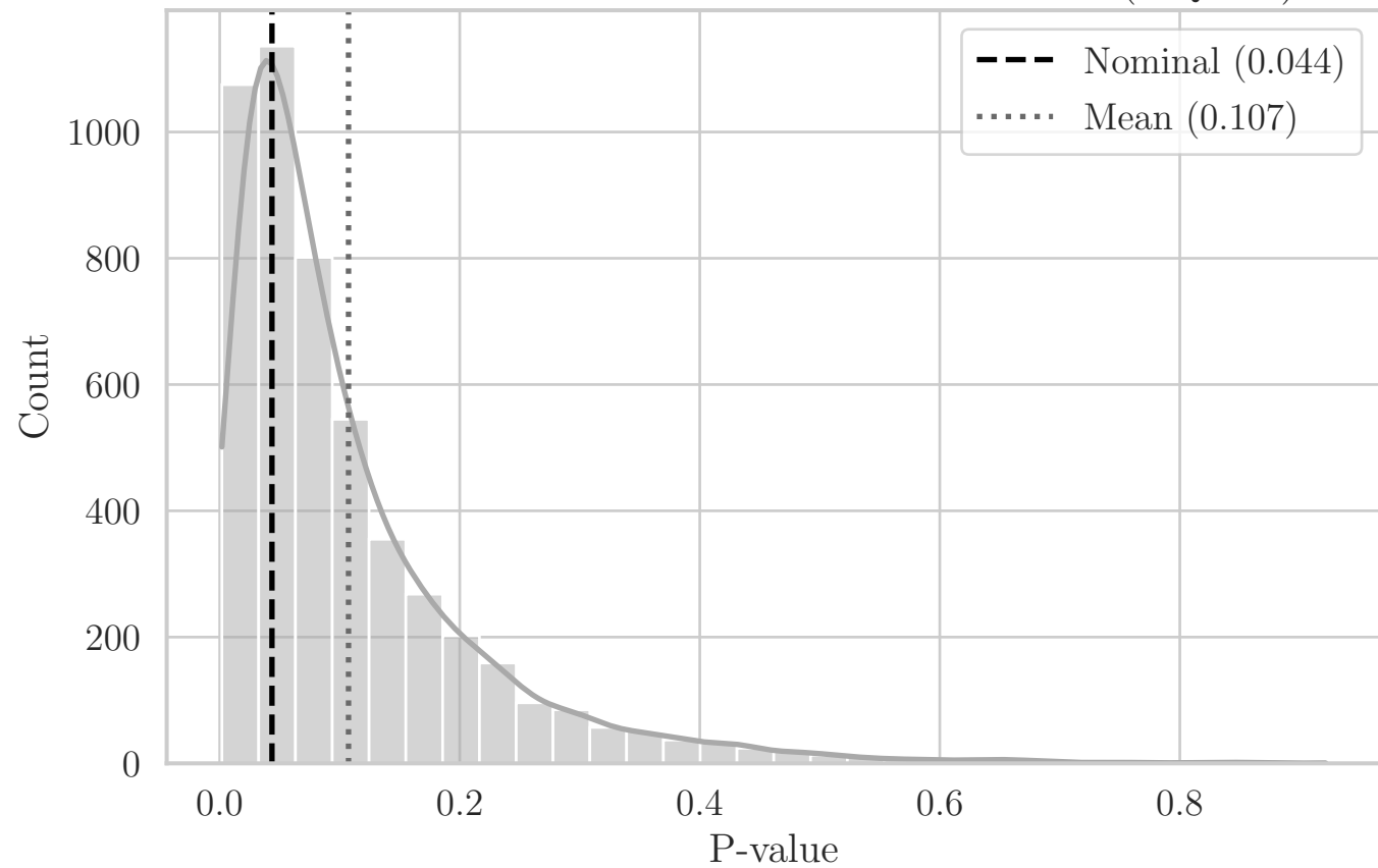
MC Distribution of P-values for ST Area_Hull (OQ XY)
