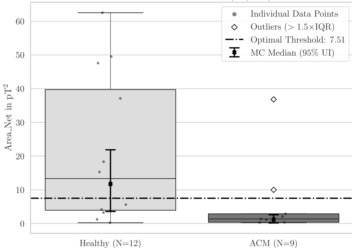
Box Plot for ST Area_Net (OQ XY)
