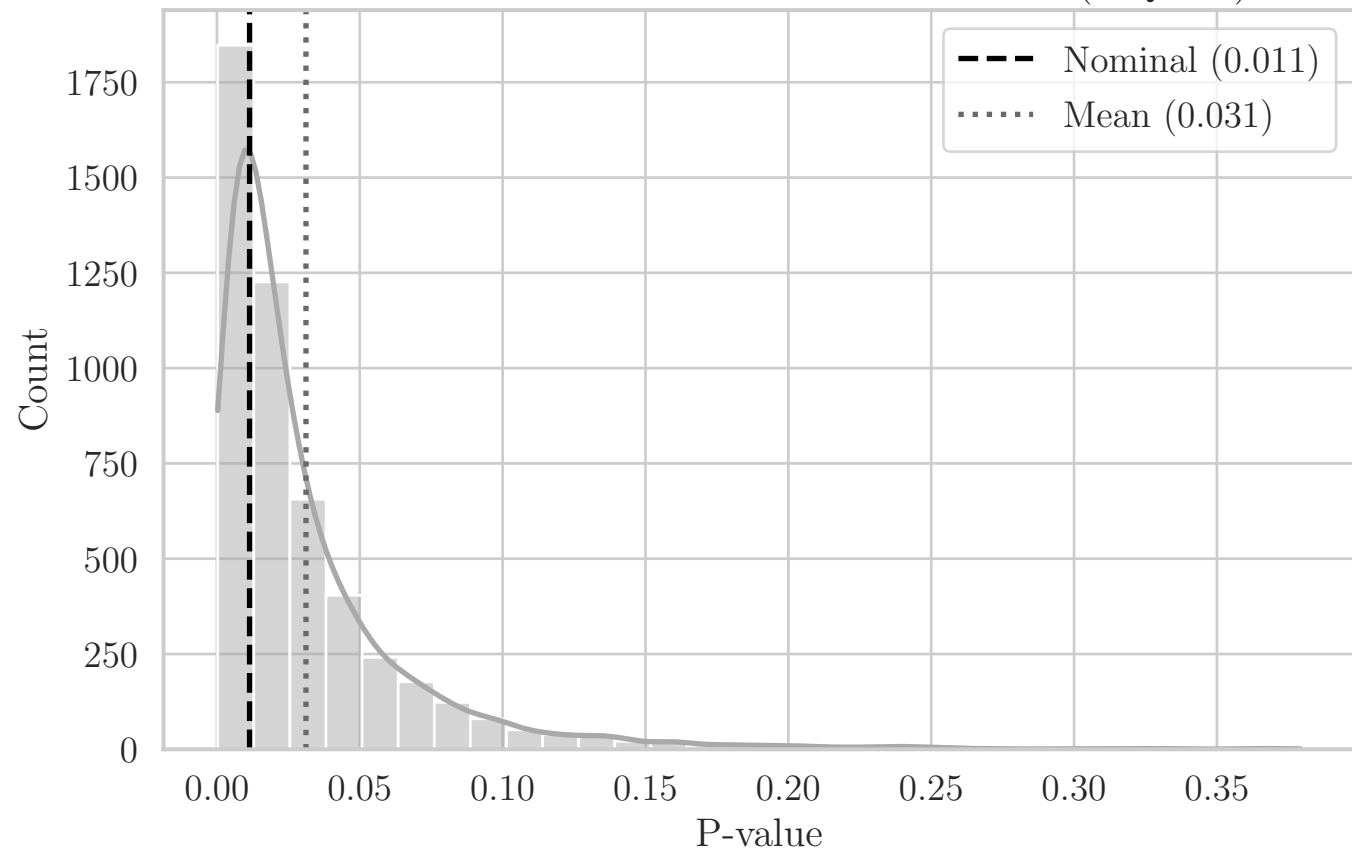
MC Distribution of P-values for T Distance (OQ XY)
