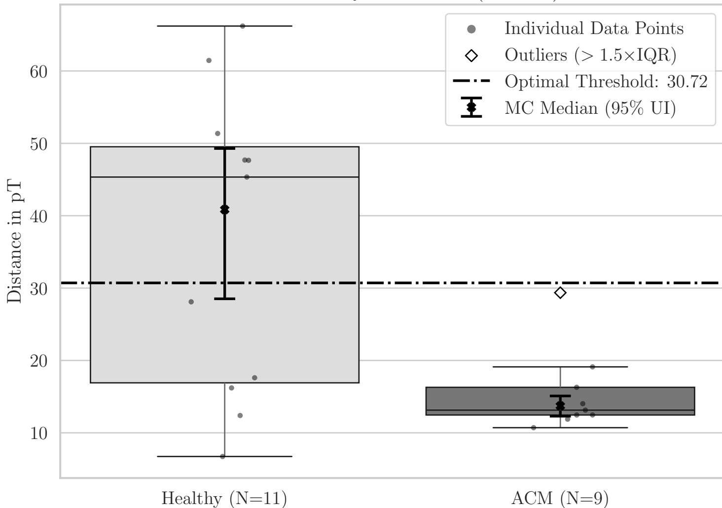
Box Plot for QRS Distance (OR XY)
