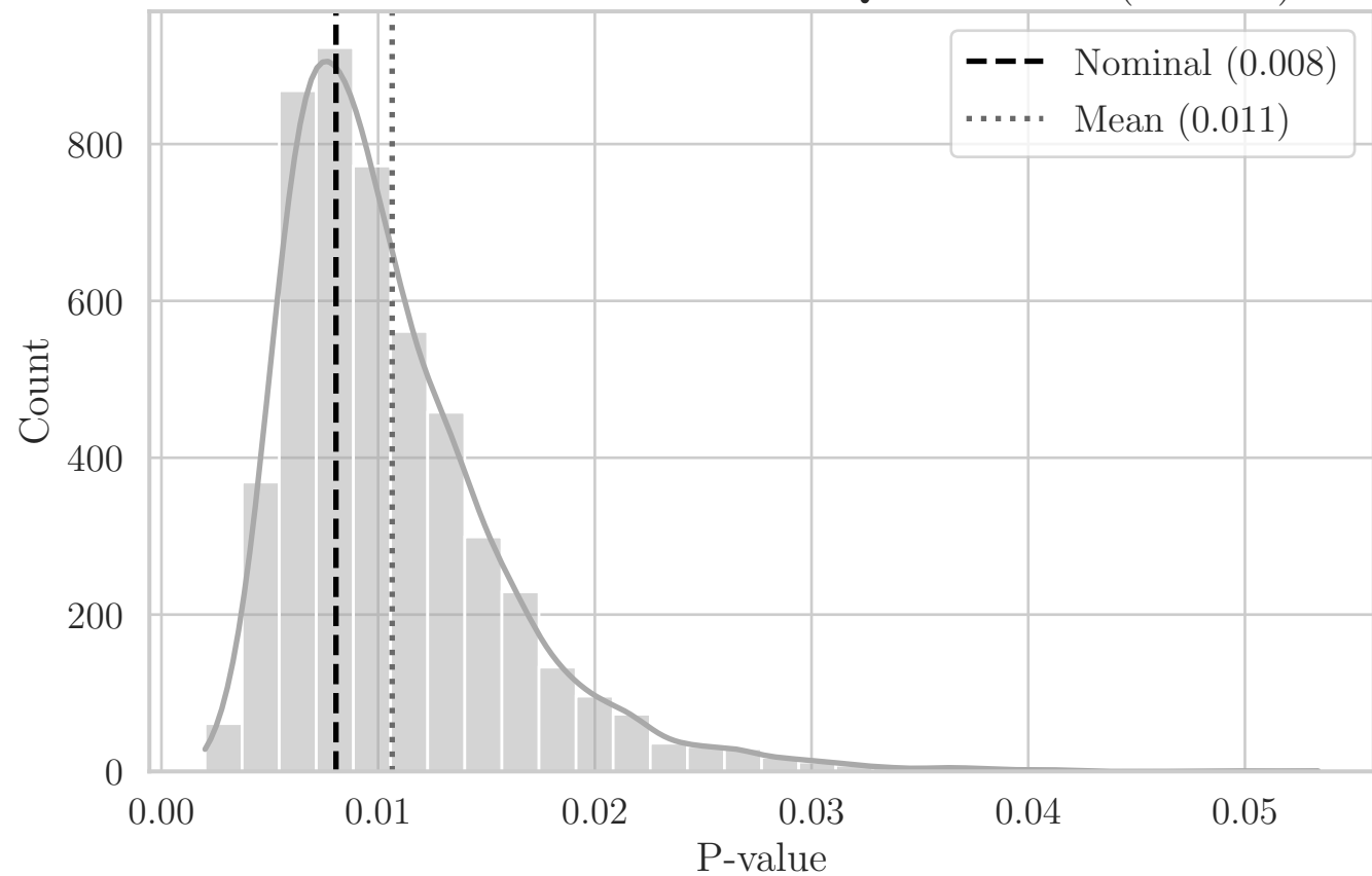
MC Distribution of P-values for QRS Distance (OR XY)
