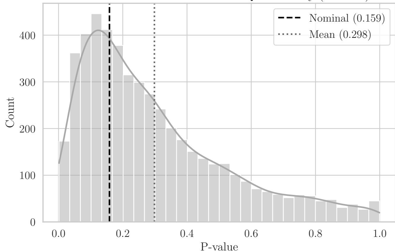
MC Distribution of P-values for QRS Solidity (OR XY)
