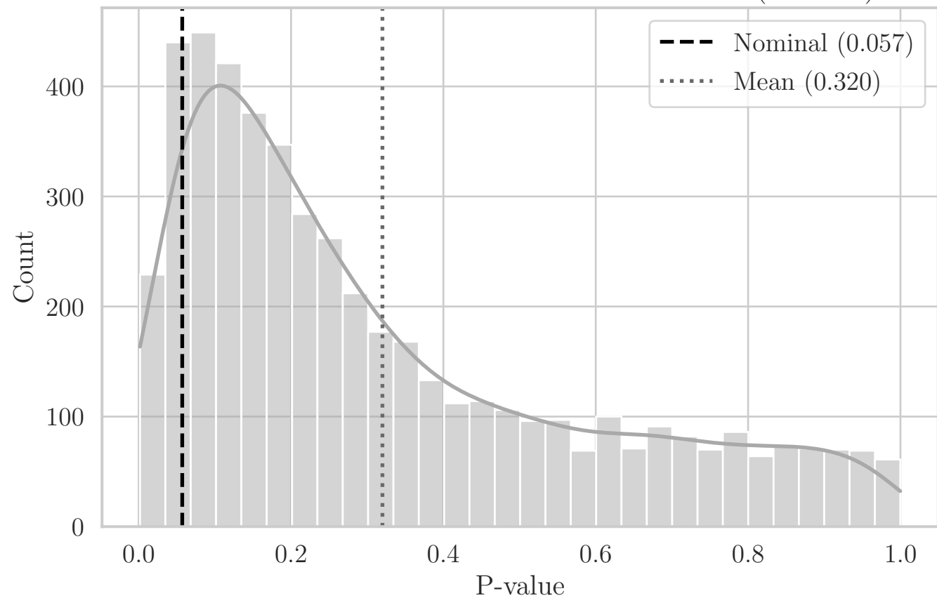
MC Distribution of P-values for ST Area_Net (OR XY)
