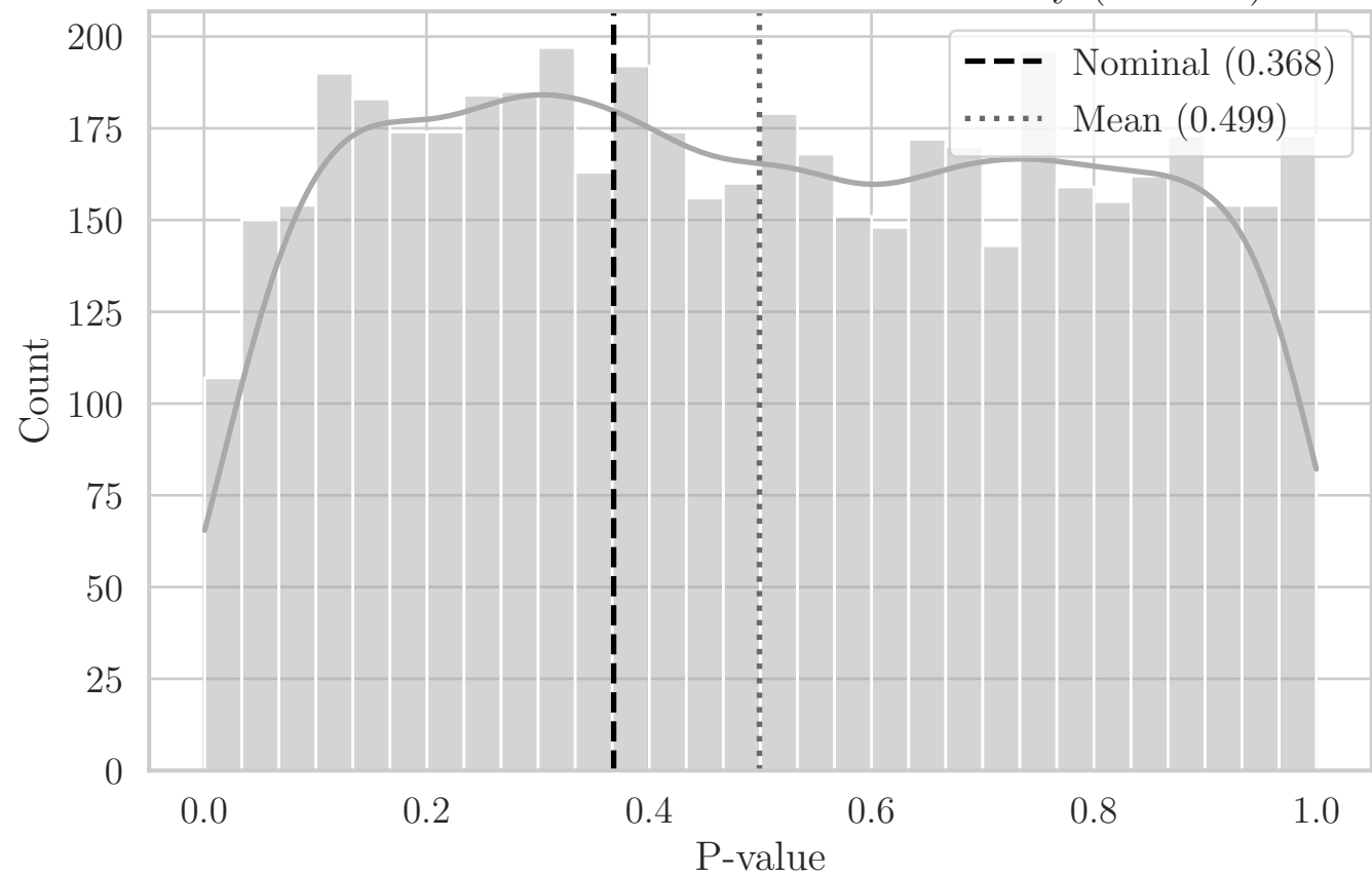
MC Distribution of P-values for ST Solidity (OR XY)
