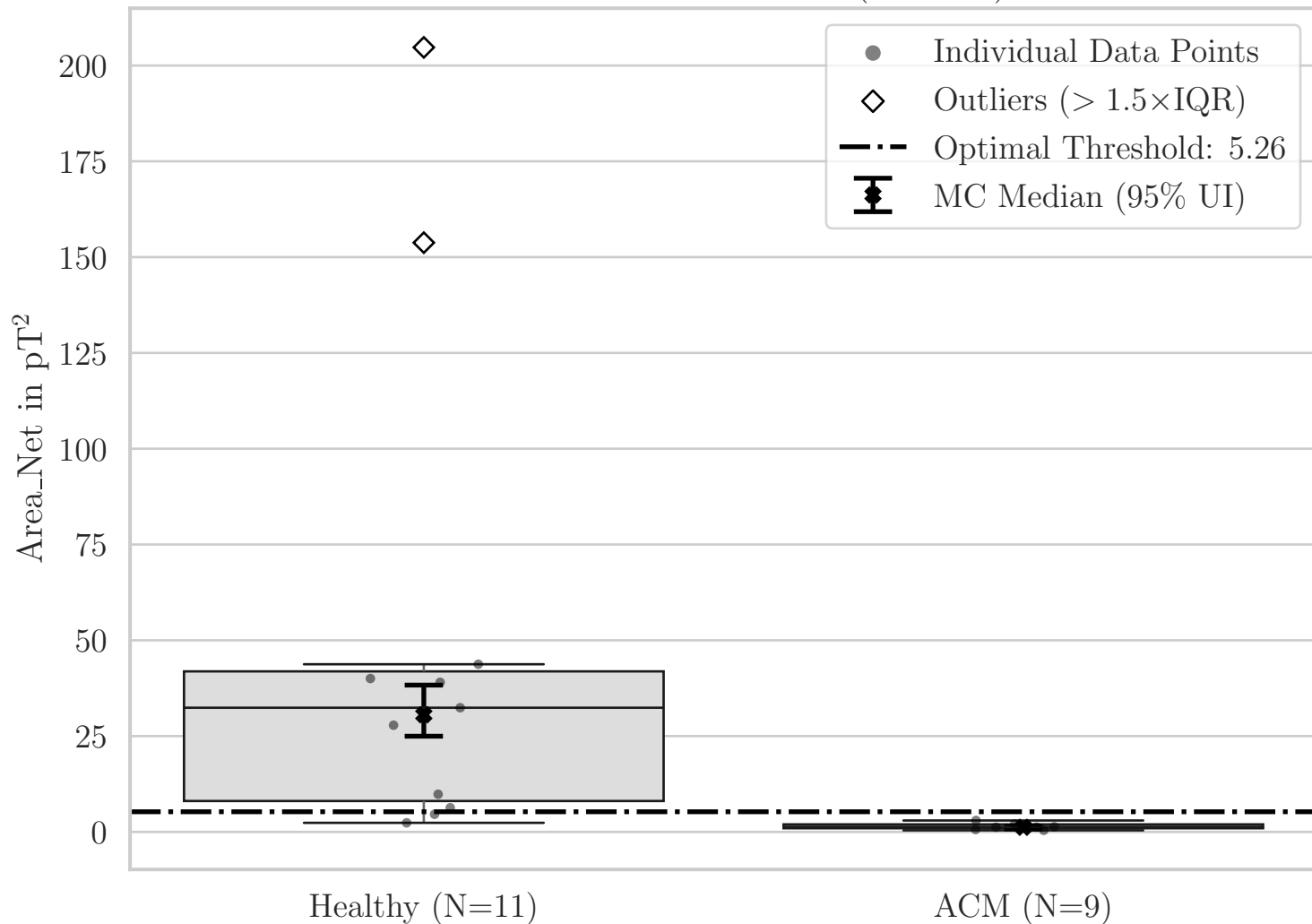
Box Plot for T Area_Net (OR XY)
