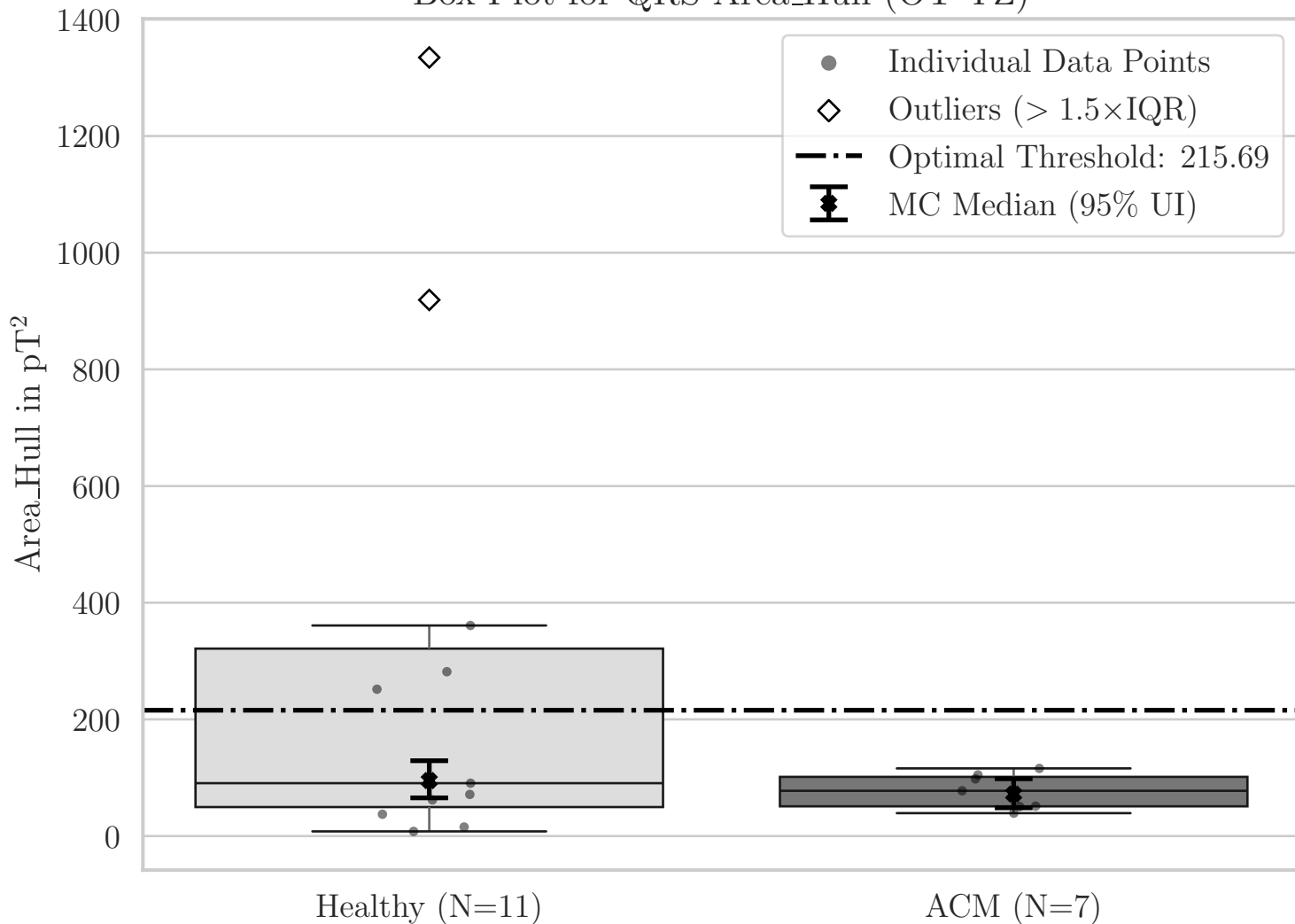
Box Plot for QRS Area_Hull (OT YZ)
