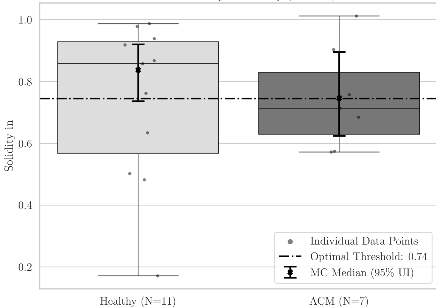
Box Plot for QRS Solidity (OT YZ)
