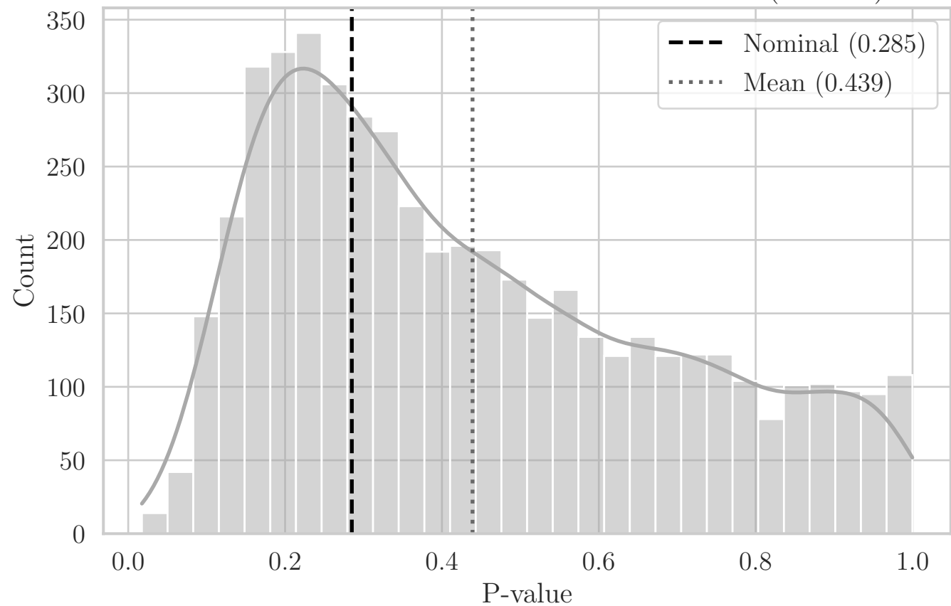
MC Distribution of P-values for ST Area_Net (OT YZ)
