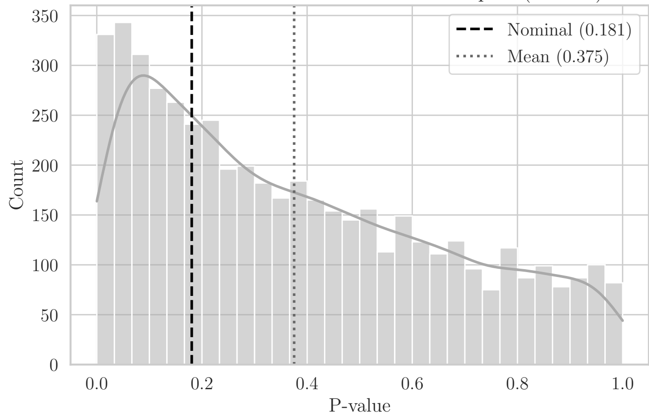
MC Distribution of P-values for ST Compact (OT YZ)
