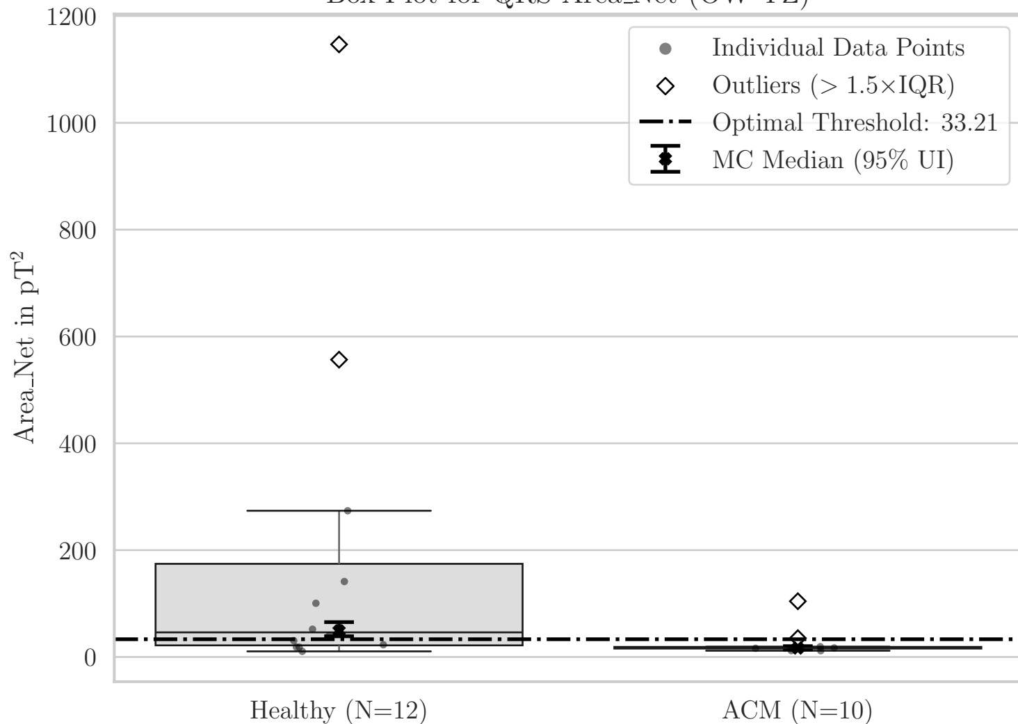
Box Plot for QRS Area_Net (OW YZ)
