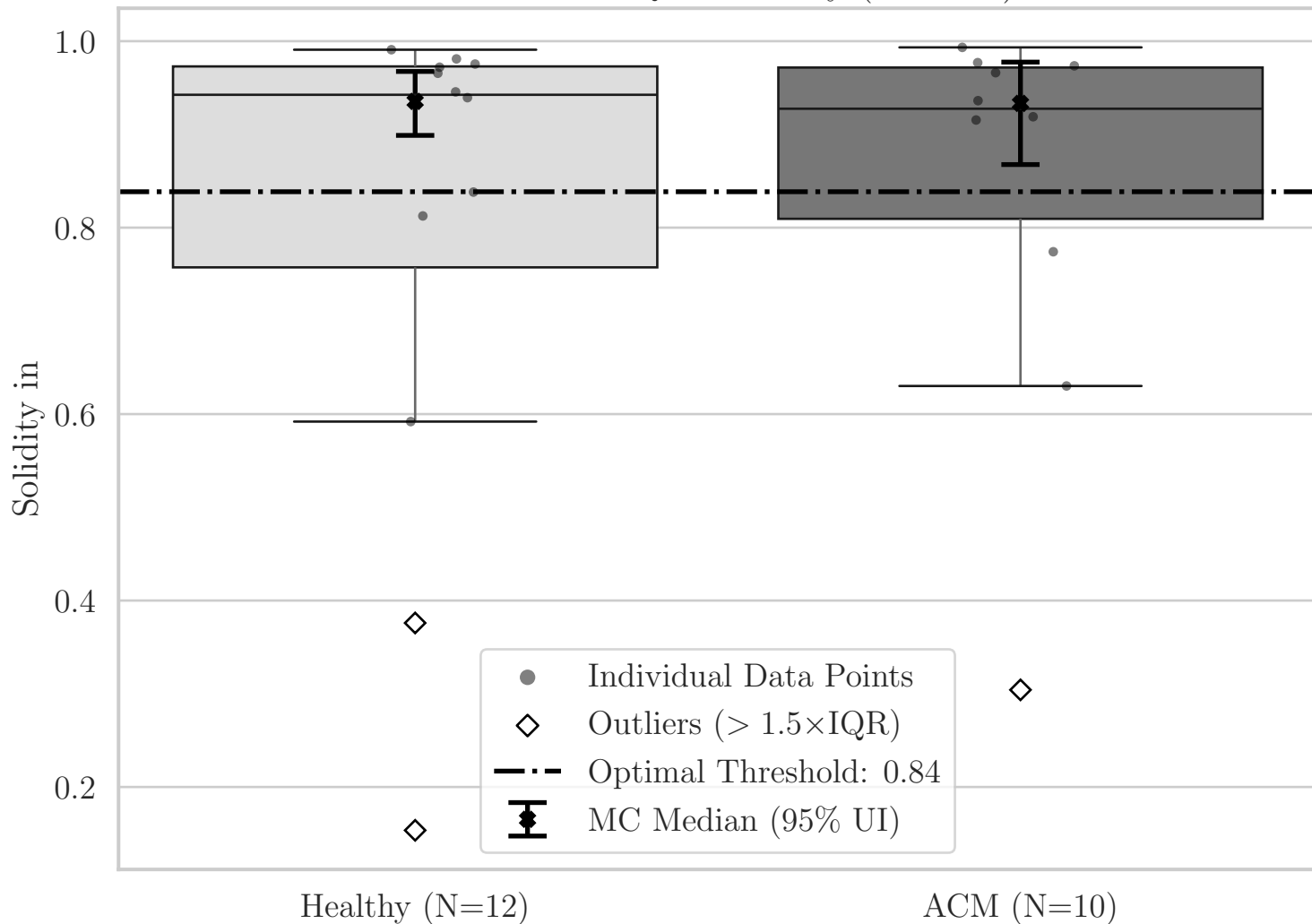
Box Plot for QRS Solidity (OW YZ)
