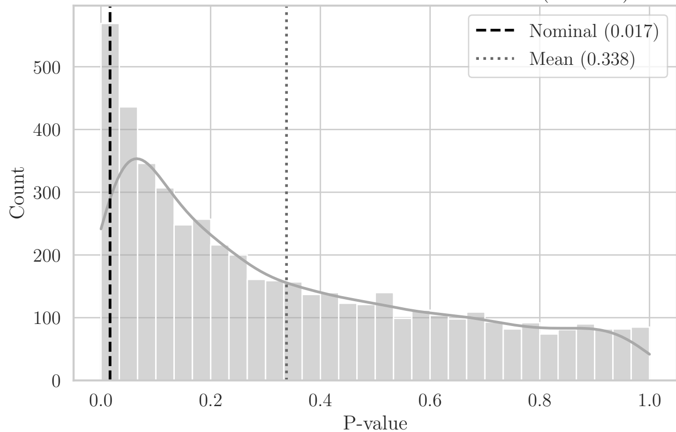
MC Distribution of P-values for ST Distance (OW YZ)
