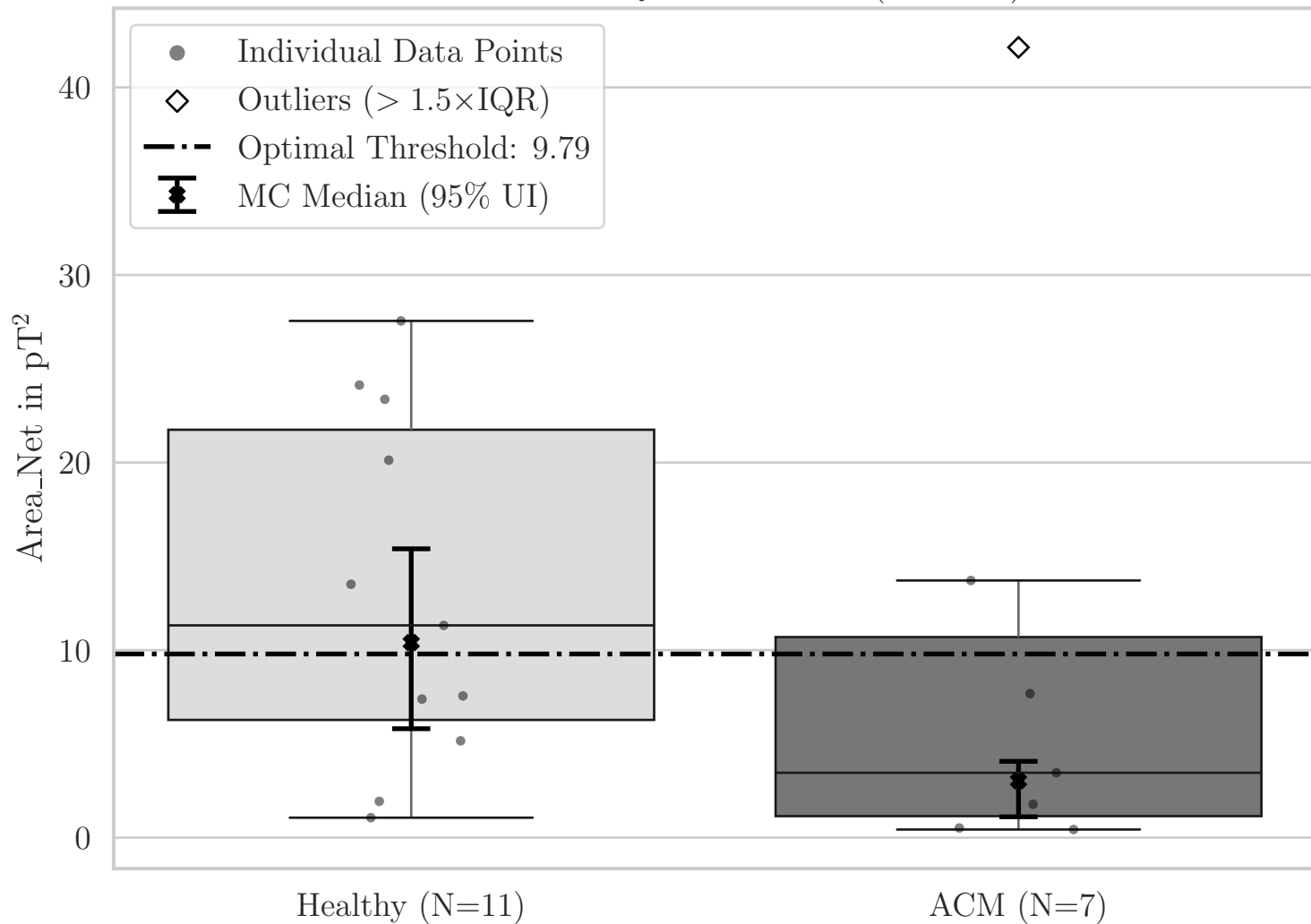
Box Plot for QRS Area_Net (OX XY)
