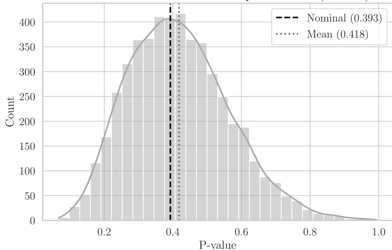
MC Distribution of P-values for QRS Distance (OX XY)
