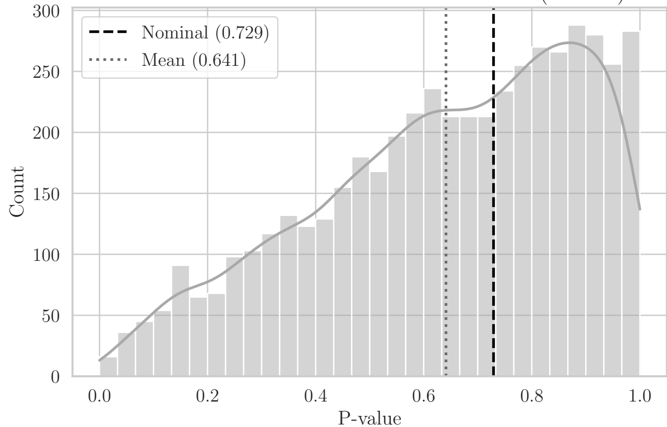
MC Distribution of P-values for ST Area_Hull (OX XY)
