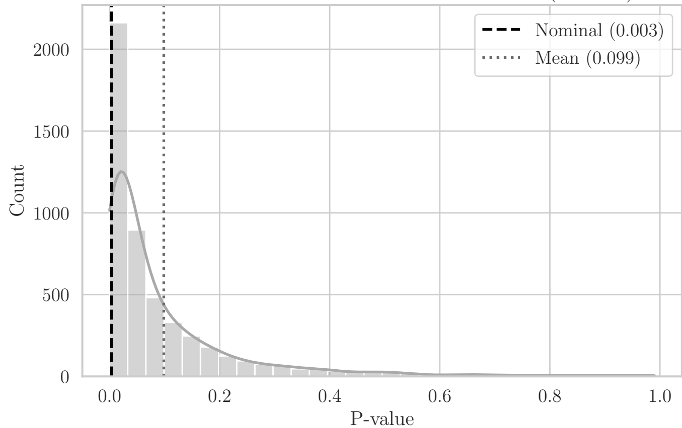
MC Distribution of P-values for ST Distance (OX XY)
