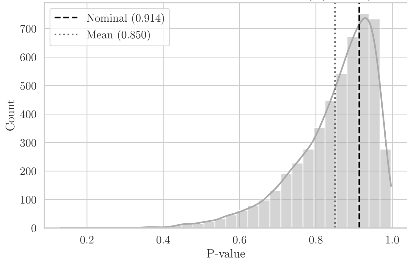
MC Distribution of P-values for T Solidity (OX XY)
