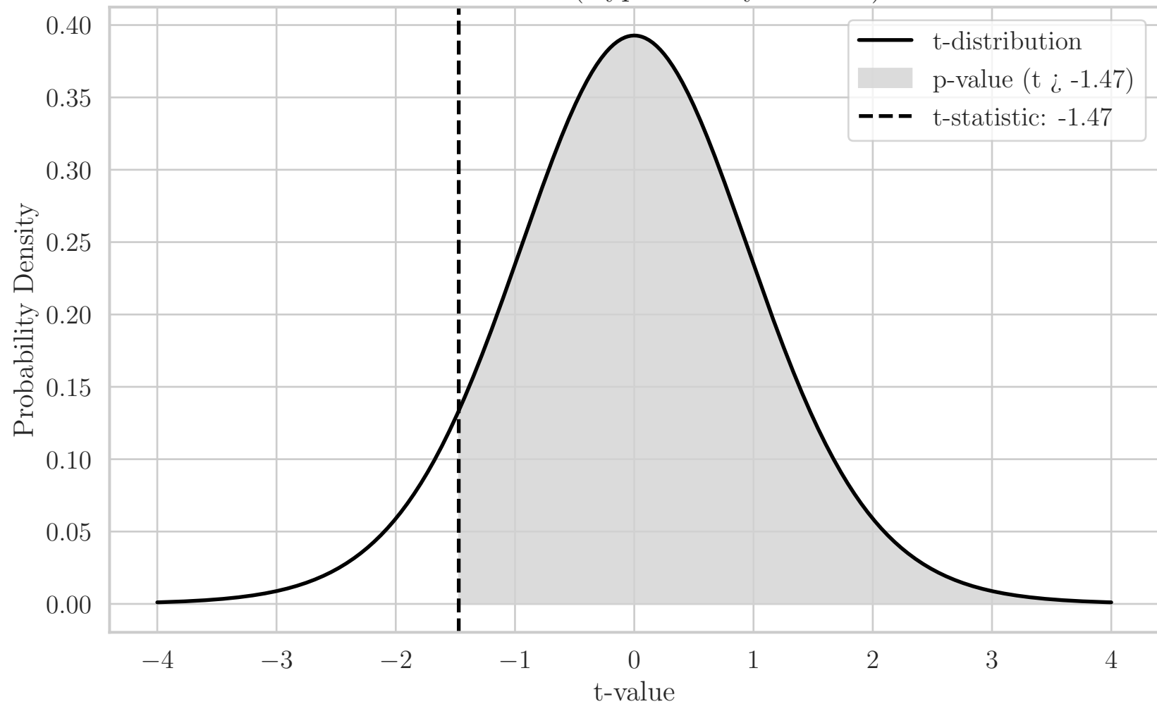
t-Distribution (Hyp: Healthy > ACM)
