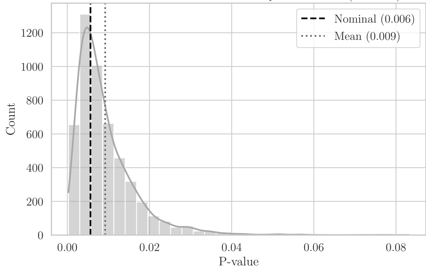
MC Distribution of P-values for QRS Distance (OY XY)
