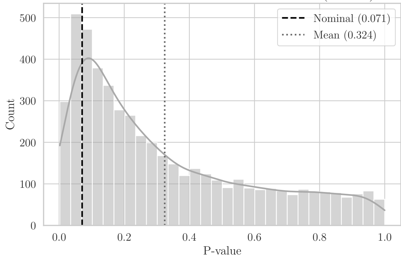
MC Distribution of P-values for ST Area_Net (OY XY)
