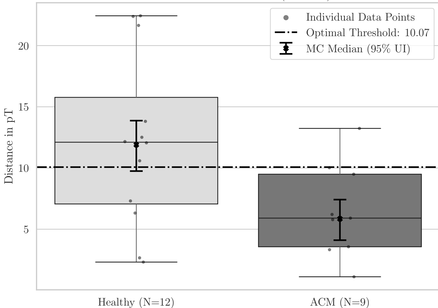
Box Plot for T Distance (OY XY)
