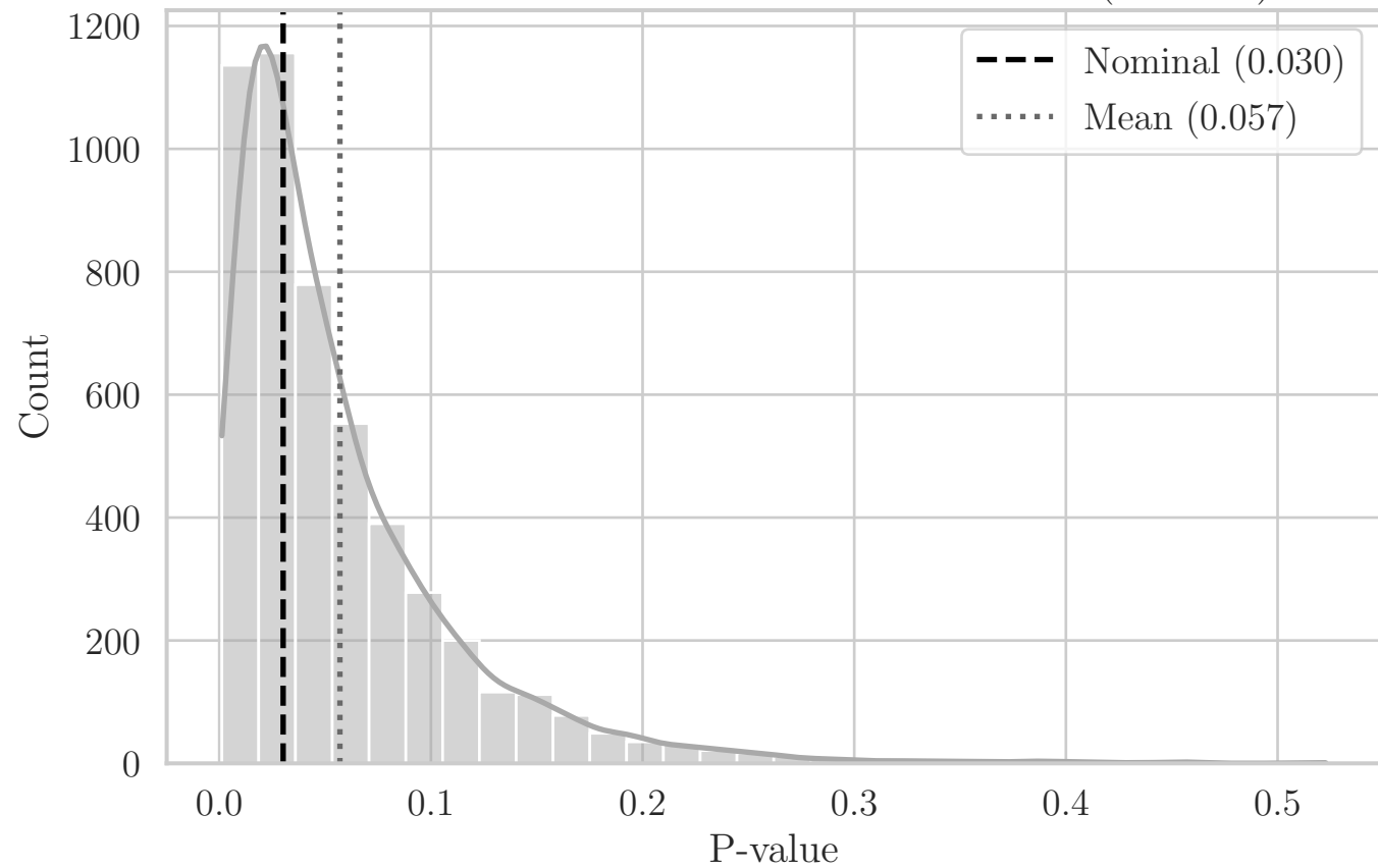
MC Distribution of P-values for T Distance (OY XY)
