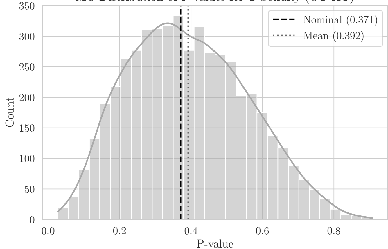
MC Distribution of P-values for T Solidity (OY XY)
