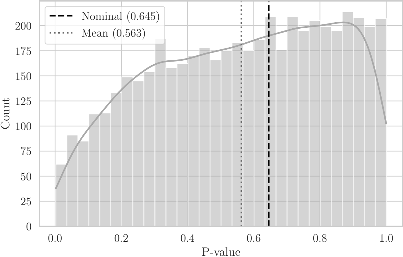
MC Distribution of P-values for ST Solidity (Aggregated Bottom-Left Quadrant YZ)
