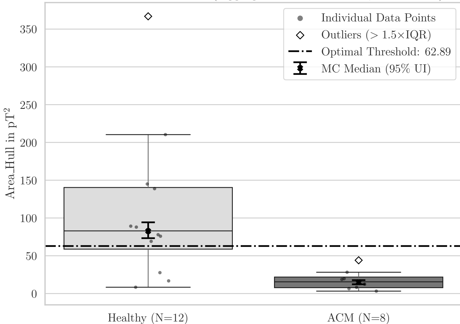
Box Plot for T Area_Hull (Aggregated Bottom-Left Quadrant YZ)
