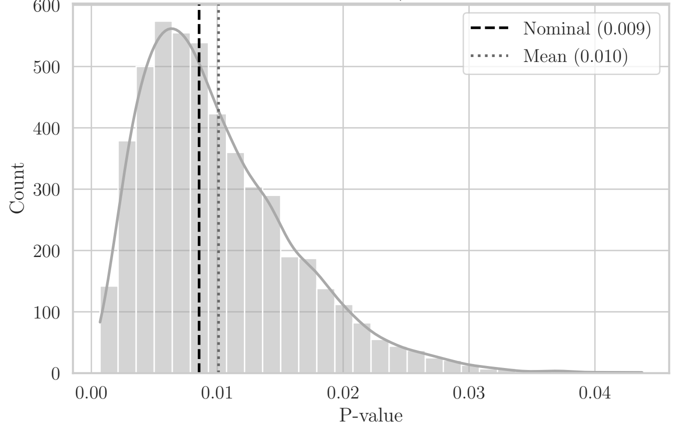
MC Distribution of P-values for T Area_Hull (Aggregated Bottom-Left Quadrant YZ)
