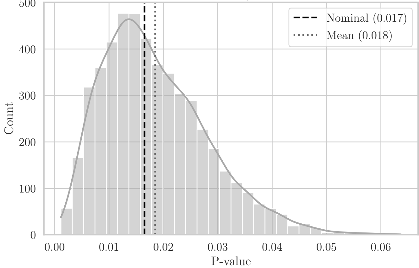
MC Distribution of P-values for T Area_Net (Aggregated Bottom-Left Quadrant YZ)
